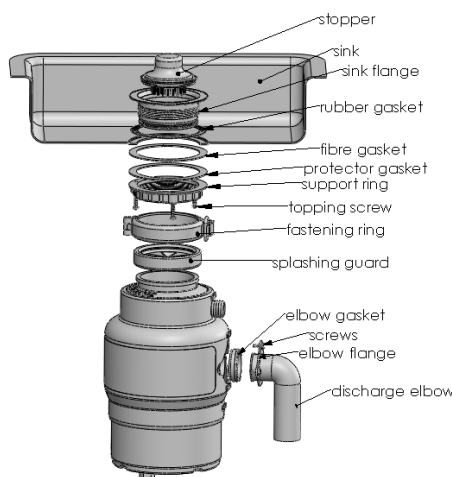
Assembly drawing
